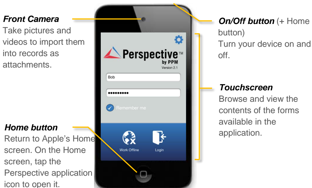
Figure 1.1: Apple Interface
