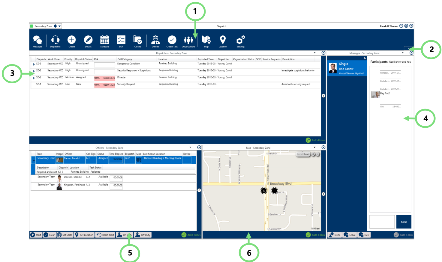
The Dispatch home screen.
